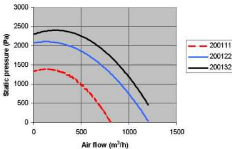
A fans Static pressure vs. Air flow
